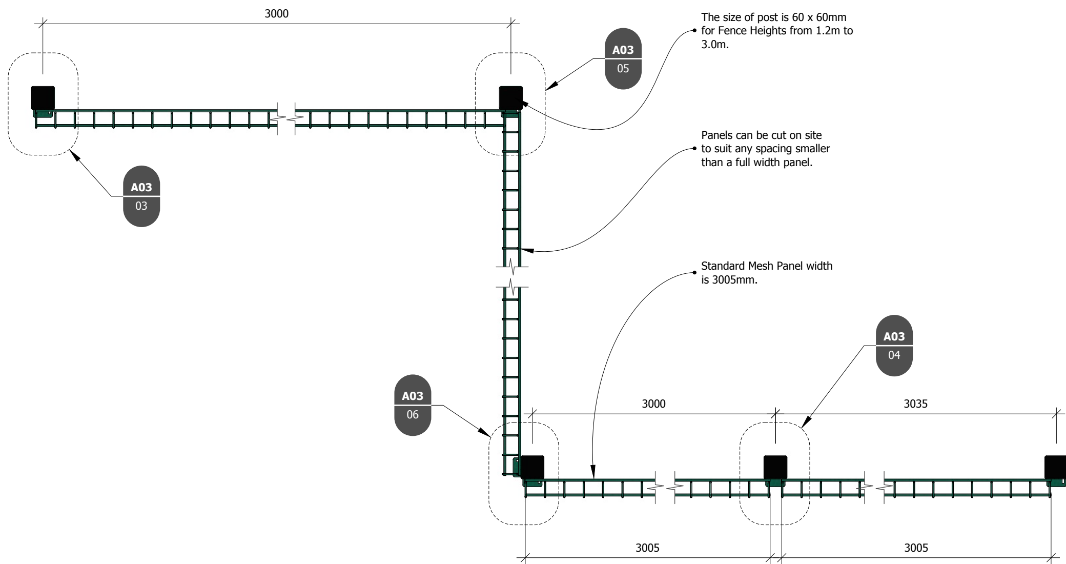
TYPICAL ASSEMBLY - PLAN scale: 1:10
